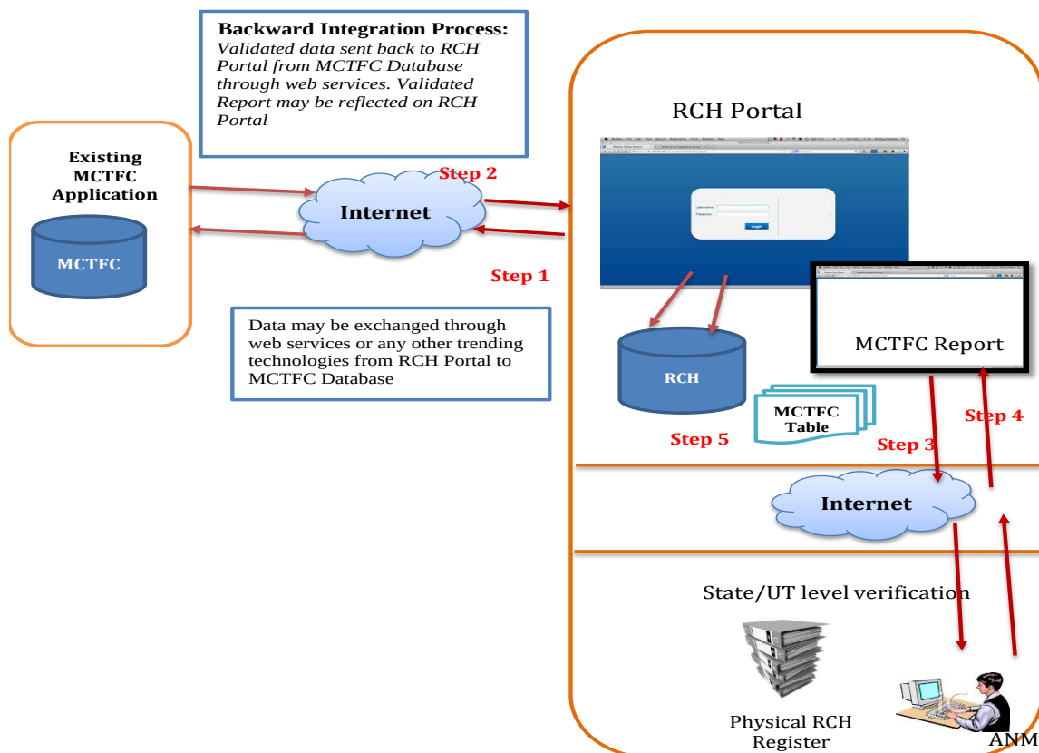
Figure1. High level diagram representing the existing MCTFC and RCH Portal Integration Flow
